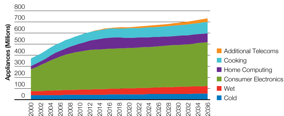
Figure 40 Gone Green number of appliances by type
