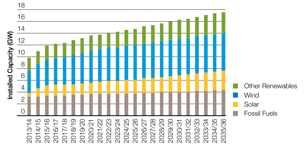
Figure 96 No Progression distributed generation installed capacity
