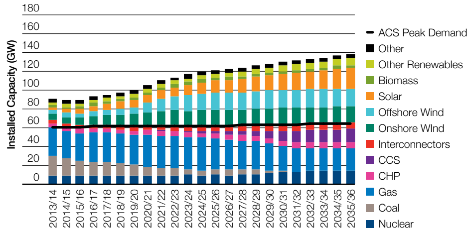
Figure 87 Low Carbon Life generation background
