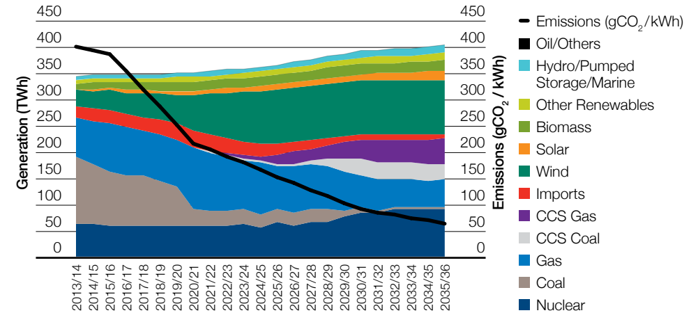
Figure 88 Low Carbon Life generation output
