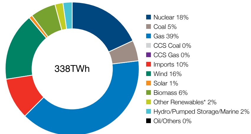
Figure 78 Slow Progression 2020/21 power generation output
