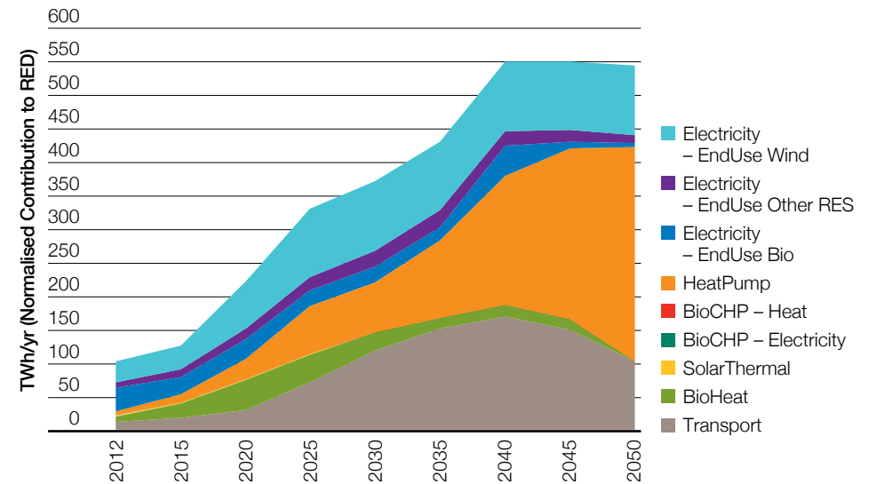
Figure 140 Low Carbon Life contributions to RED targets
