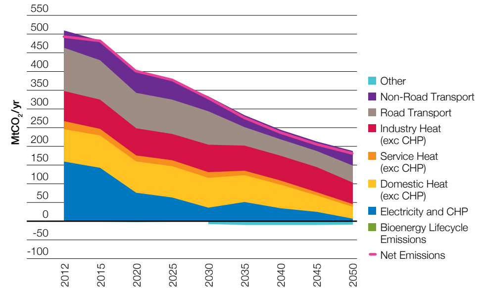
Figure 134 Slow Progression emissions by sector
