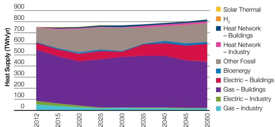
Figure 29 No Progression heat supply to 2050
