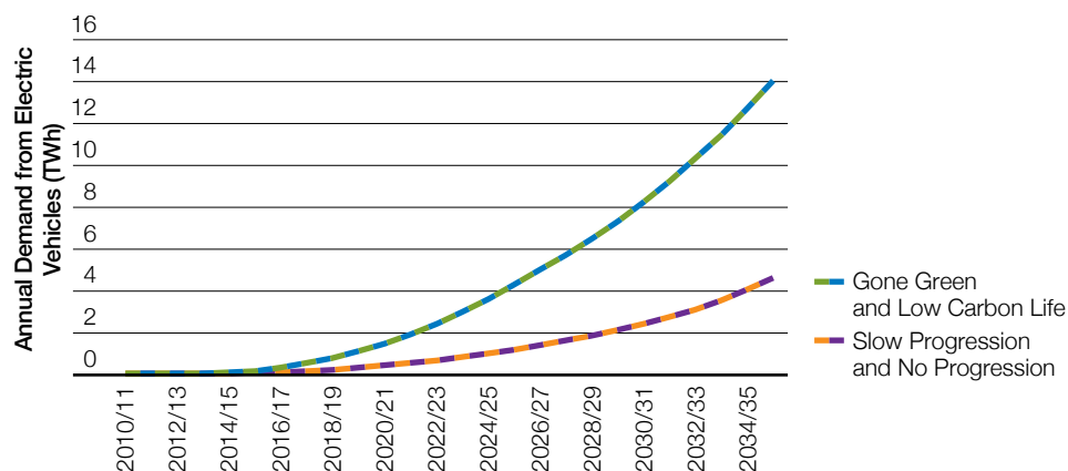
Figure 46 Annual demand from electric vehicles
