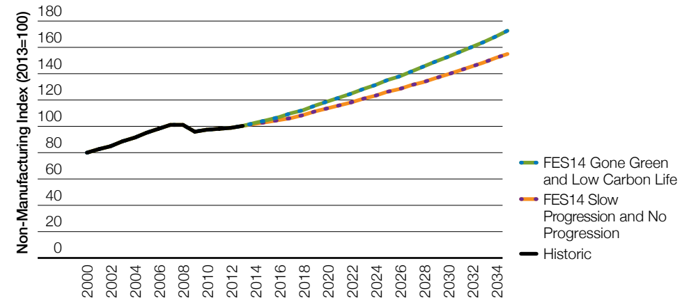
Figure 5 Indexed non-manufacturing output
