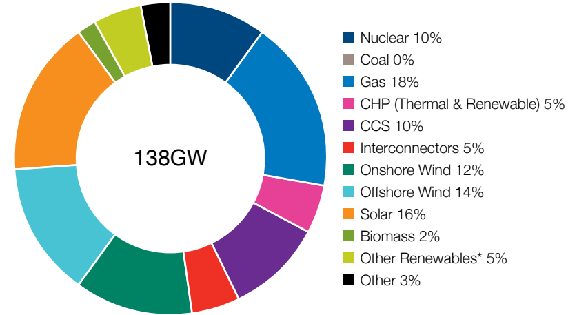
Figure 91 Low Carbon Life 2035/36 power generation capacity
