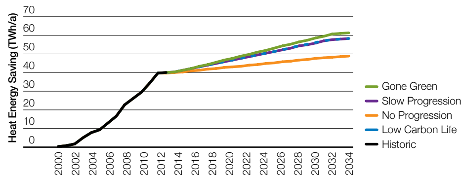
Figure 16 Total residential insulation savings by scenario (note that Low Carbon Life and Slow Progression are comparable)
