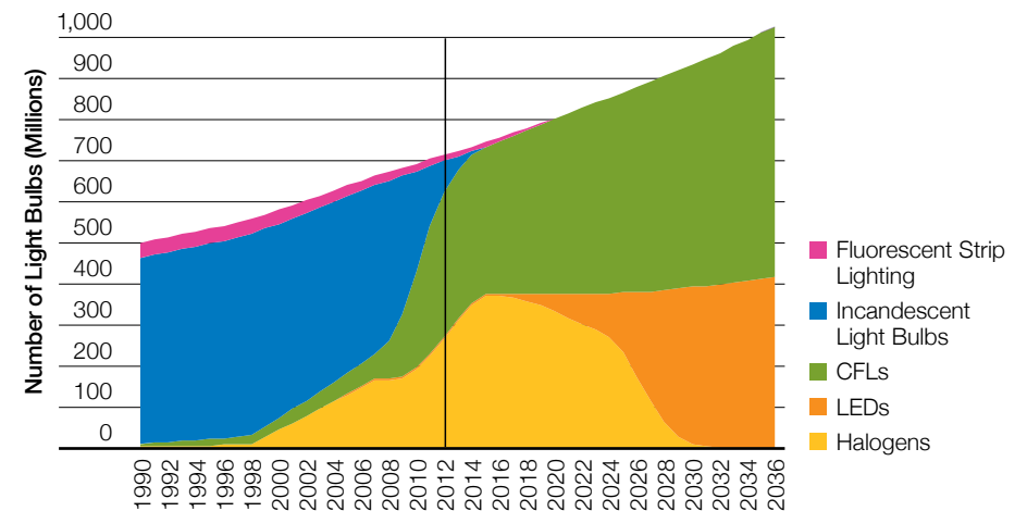
Figure 37 Residential lighting technology – Slow Progression
