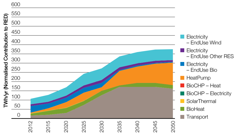
Figure 139 No Progression contributions to RED targets
