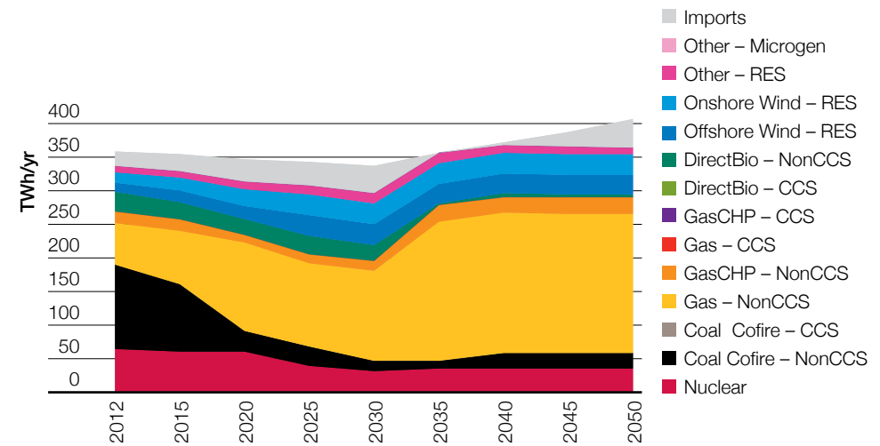
Figure 105 No Progression electricity generation to 2050
