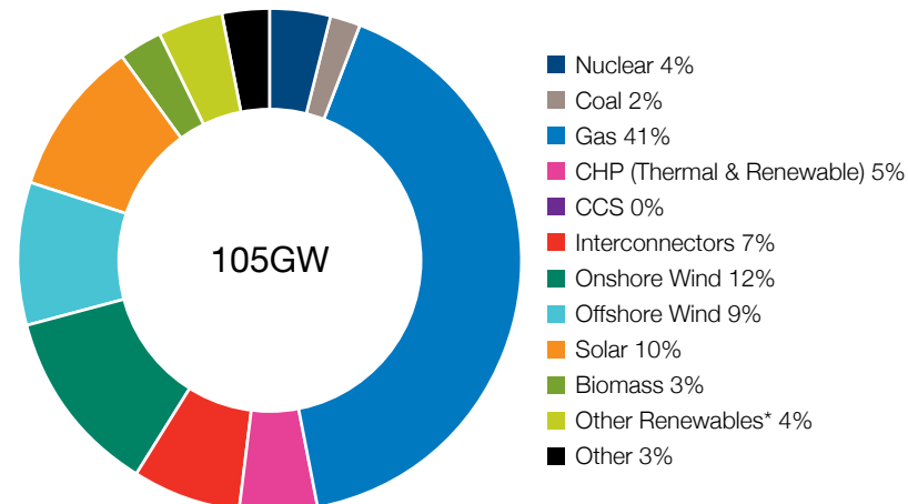
Figure 85 No Progression 2035/36 power generation capacity
