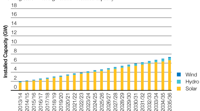
Figure 100 No Progression micro-generation installed capacity
