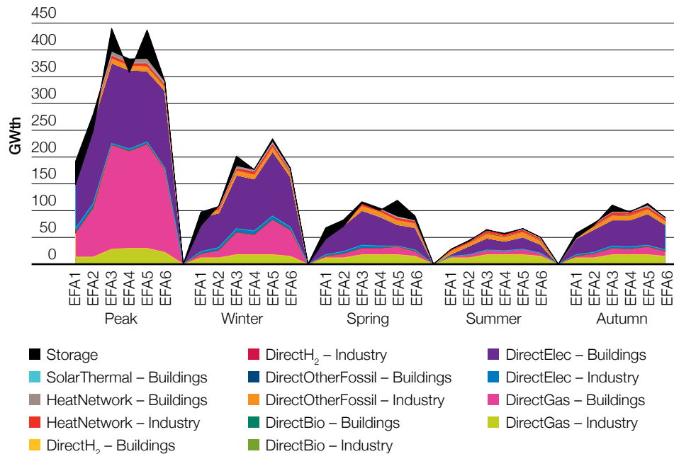
Figure 32 Heat duration supply curve for 2050
