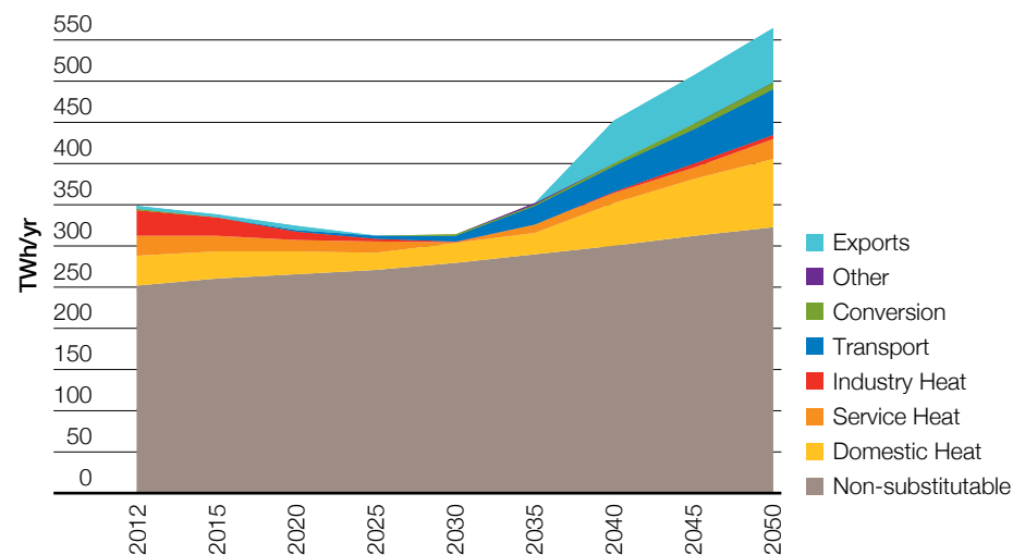
Figure 58 Gone Green electricity use to 2050
