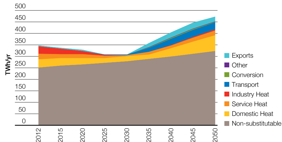
Figure 59 Slow Progression electricity use to 2050
