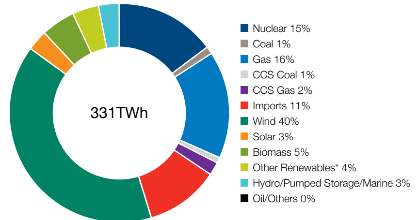
Figure 80 Slow Progression 2035/36 power generation output
